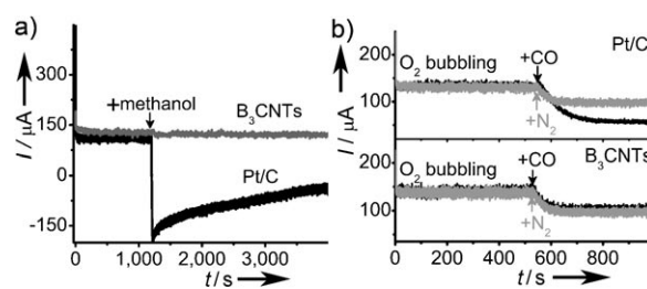
Figure 3. Chronoamperometric responses in the \text{O}_2 -saturated electrolyte for Pt/C (black) and \text{B}_3\text{CNT} (dark gray) catalysts. a) Methanol crossover tests by introducing 1.5 mL methanol into the electrolyte at 1200 s. b) CO poisoning tests by introducing additional CO with the same flow of \text{O}_2 into the electrolyte at 520 s. Parallel experiments for Pt/C (40 wt% Pt loading) and \text{B}_3\text{CNT} catalysts are carried out by replacing CO with the same flow of \text{N}_2 (light gray).
